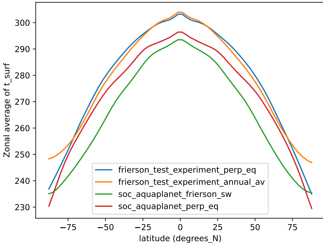
Zonal average of t_{surf} as a function of latitude
